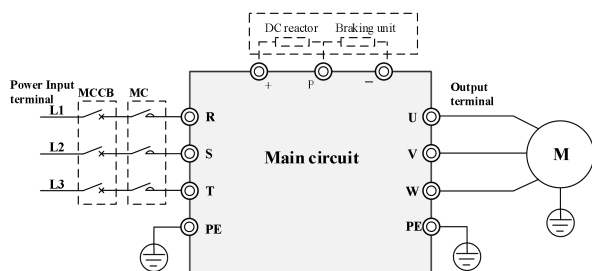
Figure 2-5-2 Main circuit wiring diagram 2
